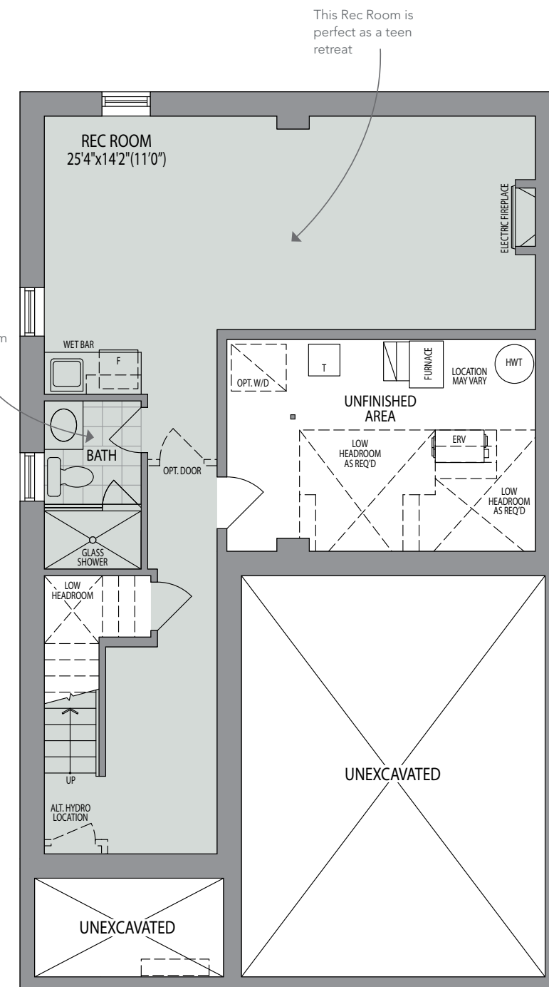
FINISHED LOWER LEVEL ELEVATION A
